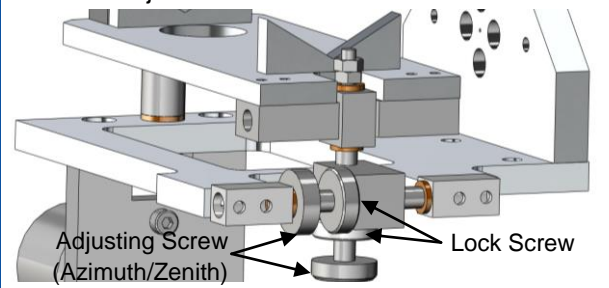
XY Axis Adjustment Unit
