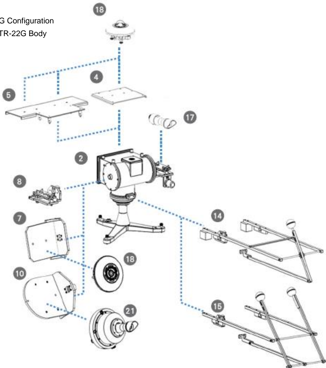
Figure 9-8. STR-21G/22G Configuration
